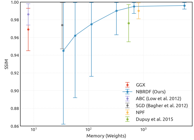
Figure 17: Average SSIM vs Memory footprint (log scale) for multiple representations of BRDFs, including standard deviations. In our method (NBRDF) the network size can be adjusted to select the reconstruction accuracy, thus we include data points for multiple sizes.
