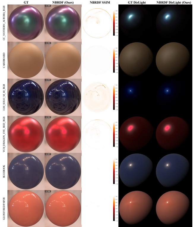
Figure 5: NBRDF reconstruction of measured materials from the RGL database [DJ18] (top 4) and from Nielsen et al. [NJR15] (bottom 2), using environment map and directional illuminations.
