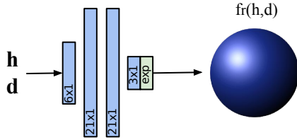
Figure 1: Diagram of a Neural-BRDF (NBRDF).
