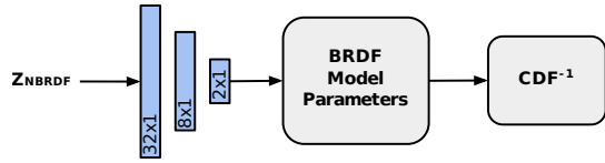
Figure 4: Scheme for quick computation of inverse CDF from an NBRDF: we train a network to map from latent NBRDF embeddings to importance sampling parameters of a chosen analytic BRDF model.
