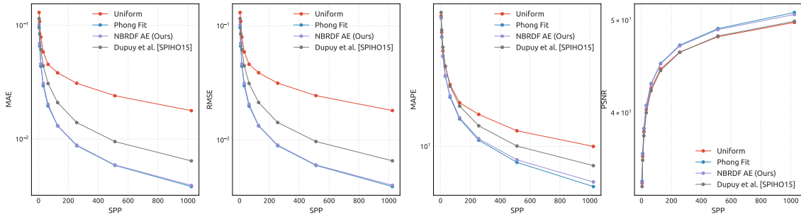
Figure 16: Average errors (log scale) vs SPP for MERL testset materials in the kitchen scene from Figure 15. Left to right : MAE, RMSE, MAPE, PSNR.
