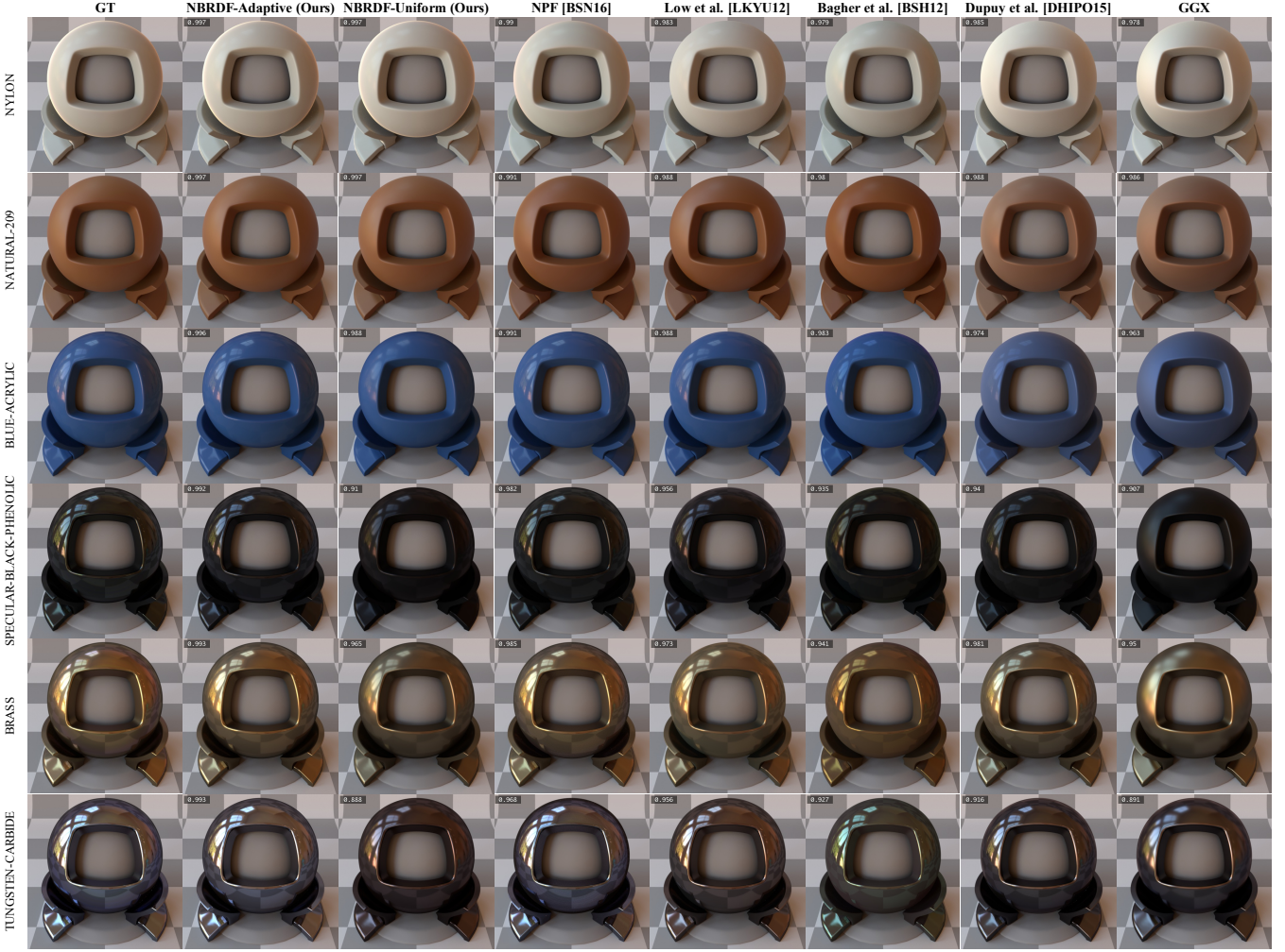
Figure 6: Reconstruction of MERL materials using different BRDF representations, including the average SSIM value for each image. For both NBRDF columns we utilised a fixed network size of 675 weights ( 6 \times 21 \times 21 \times 3 ).
